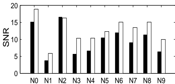
Figure 4: SNR comparison between the Bodden model (black bar) and our model (white bar). Target is at 30° and interference is at -10°.
