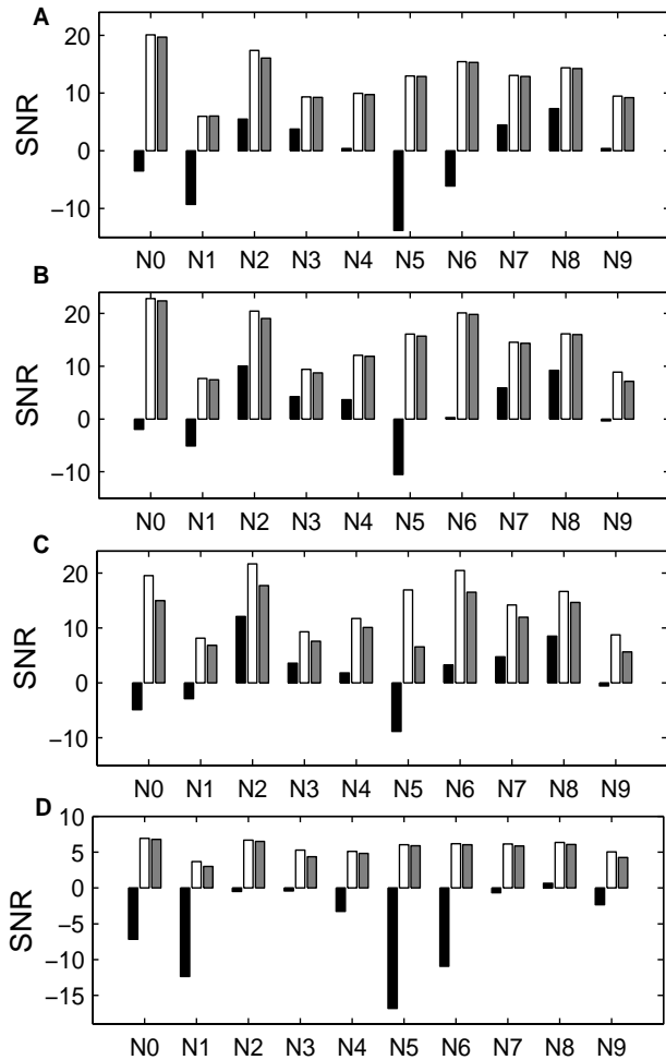
Figure 3: Systematic evaluation. Black bar represents the mixture SNR, white bar is the SNR using the ideal binary mask and gray bar corresponds to results from our system. The corpus contains 10 male utterances mixed with ten interferences (N0: pure tone; N1: white noise; N2: noise burst; N3: 'cocktail party'; N4: rock music; N5: siren; N6: trill telephone; N7: female speech; N8: male speech; N9: female speech). A: Target at 0°, interference at 5°. B: Target at 45°, interference at 50°. C: Target at 70°, interference at 75°. D: three-source configuration: target at 0°, interference at -30° and 30°.
