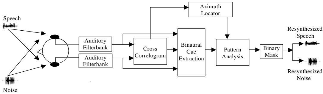
Figure 1: Schematic diagram of the model. We obtain binaural signals by convolving the input signals with head related impulse responses (HRIR). A psychoacoustically motivated auditory periphery is simulated: cochlear filtering, half-wave rectification to simulate auditory nerve firing, low pass filtering for evaluating envelopes at high frequencies and square root to simulate saturation effects. Azimuth localization is based on the cross-correlation mechanism. We compute local ITD and IID independently for all frequency channels. A decision block produces an estimation of the ideal binary mask. The resynthesis path allows the reconstruction of the target signal.
