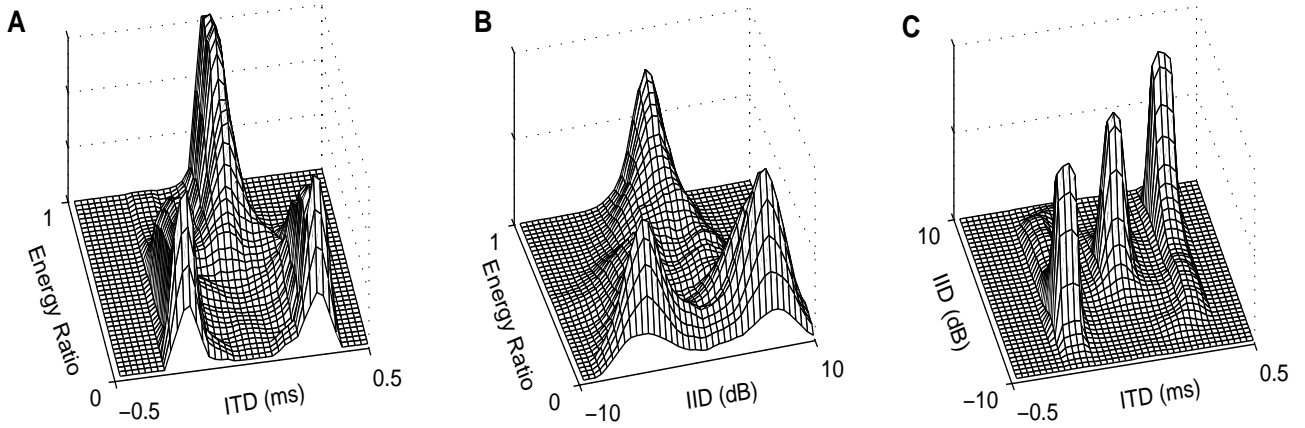
Figure 2: A: Relationship between ITD and the energy ratio. B: Relationship between IID and the energy ratio. C: Clustering in the ITD-IID feature space. Histograms are obtained for speech at 0^\circ and interfering noise at 30^\circ and -30^\circ , for the channel number 85 with center frequency \sim 1.7 kHz.
